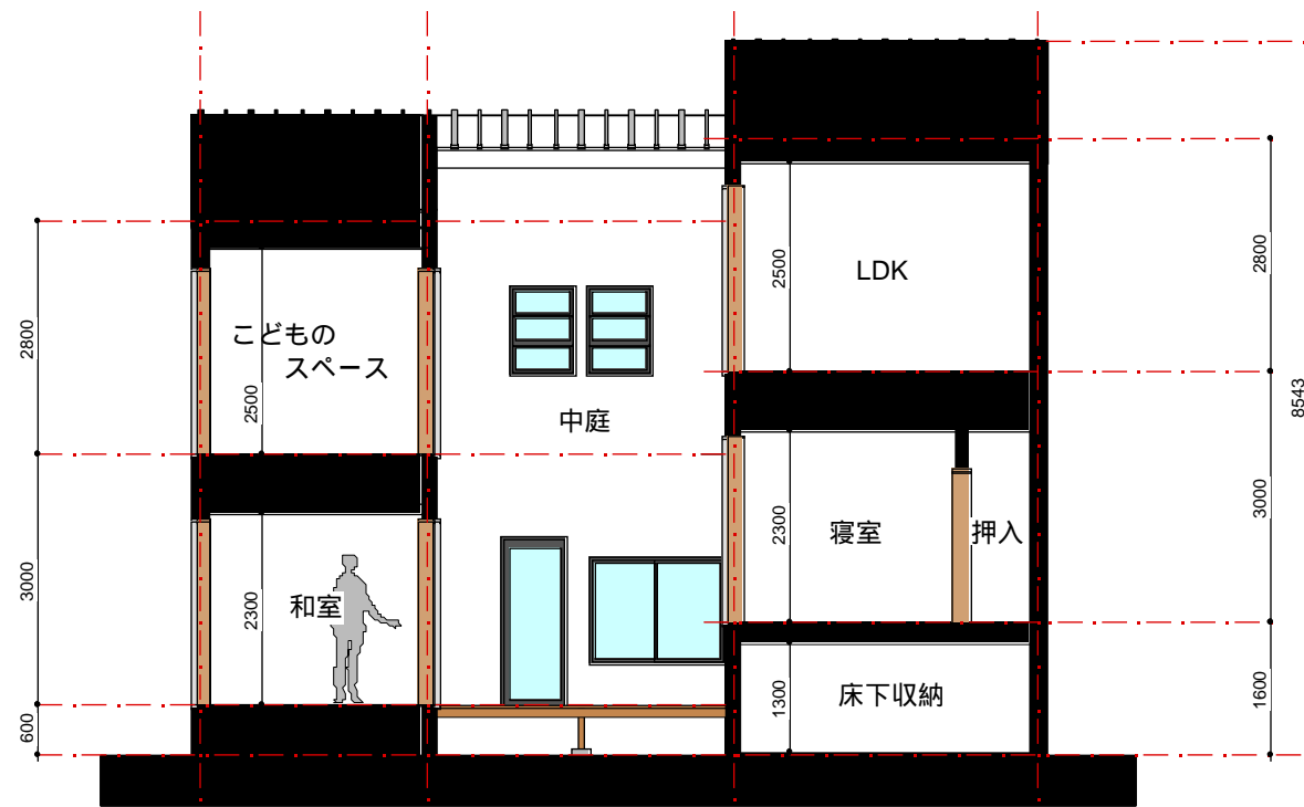
SECTION PLAN
