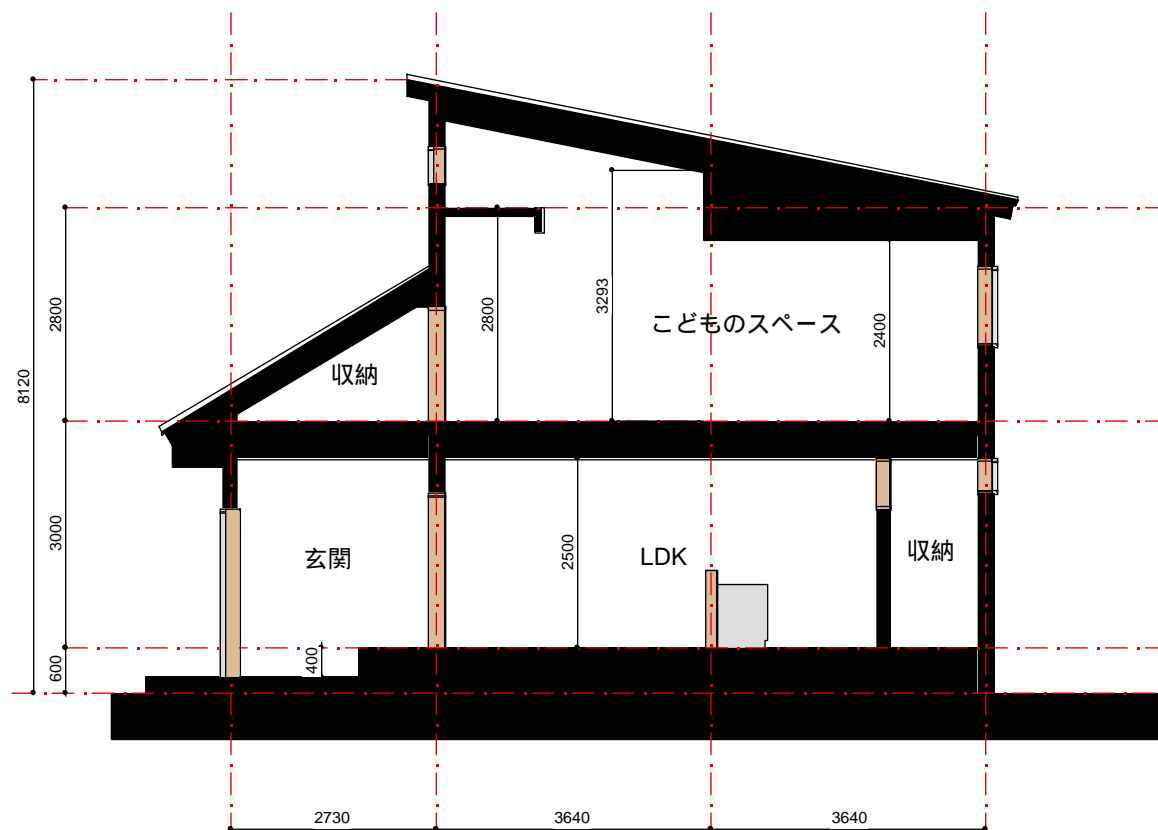
SECTION PLAN
